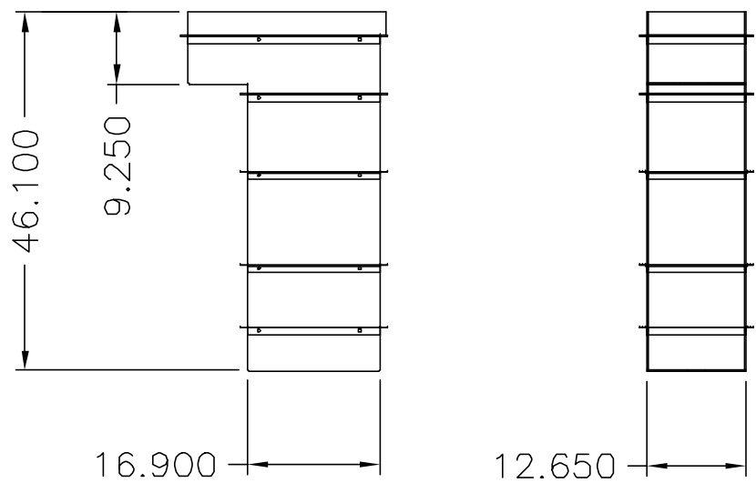
LOST CASING DIMENSIONS
