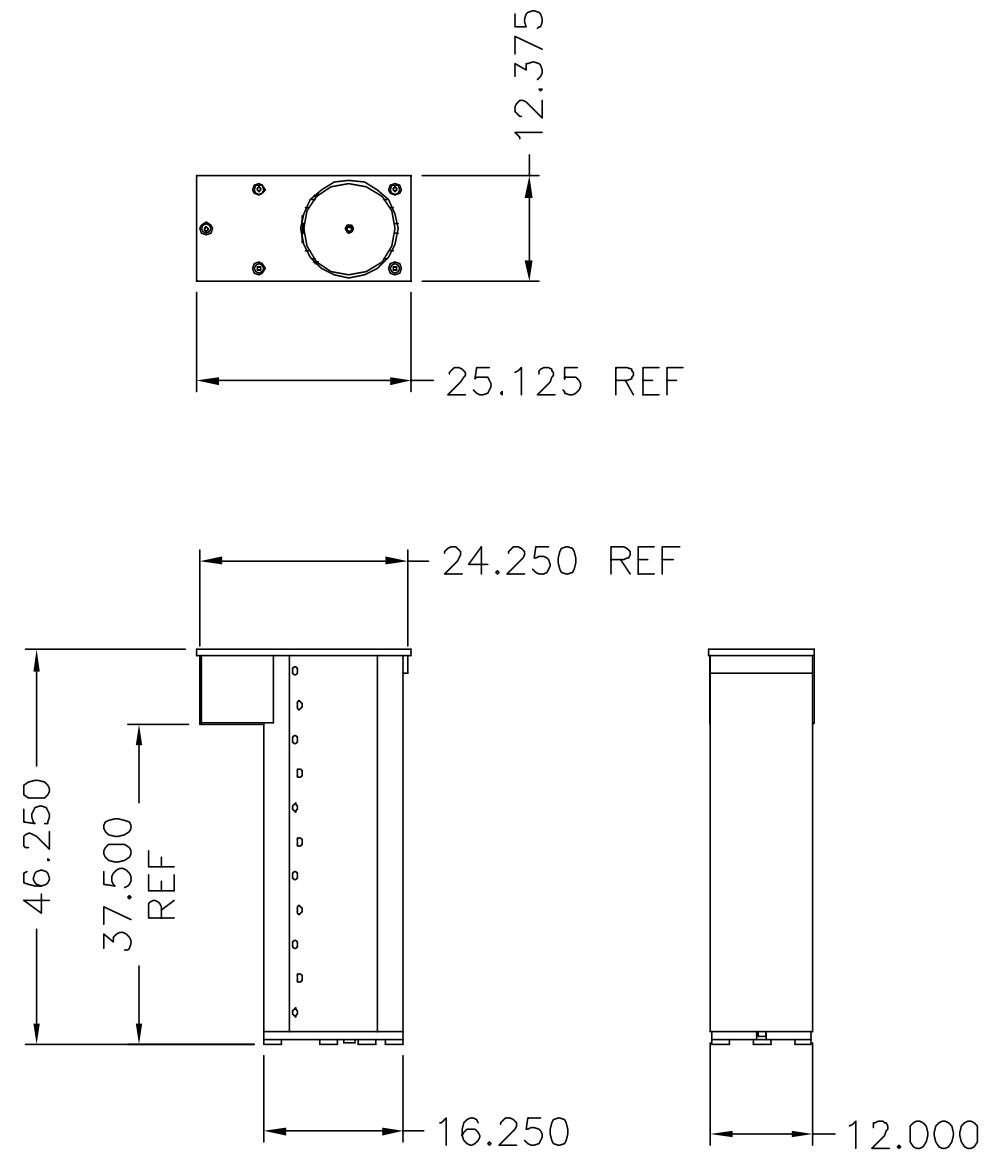
BOLLARD DIMENSIONS
